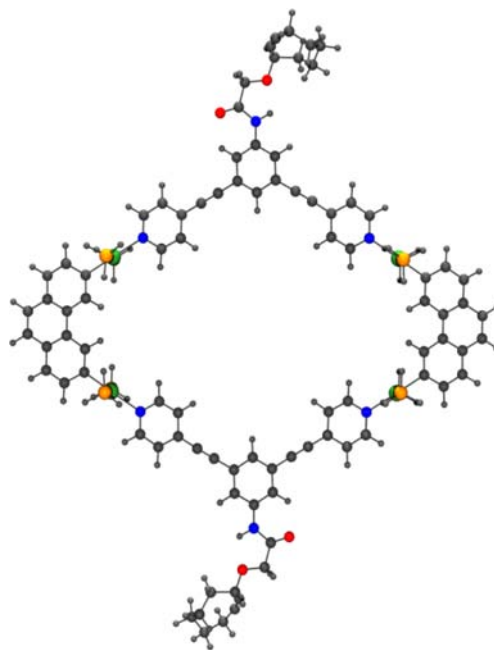
Figure 3. DFT-optimized structure of metallacyclic rhomboid 6 . Color code: gray, C; light gray, H; blue, N; red, O; orange, P; green, Pt.
