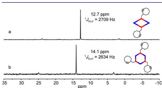
Figure 1. ^{31}\text{P}\{^1\text{H}\} NMR spectra of (a) rhomboid 6 and (b) hexagon 7 .
